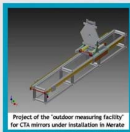
Project of the "outdoor measuring facility" for CTA mirrors under installation in Merate
